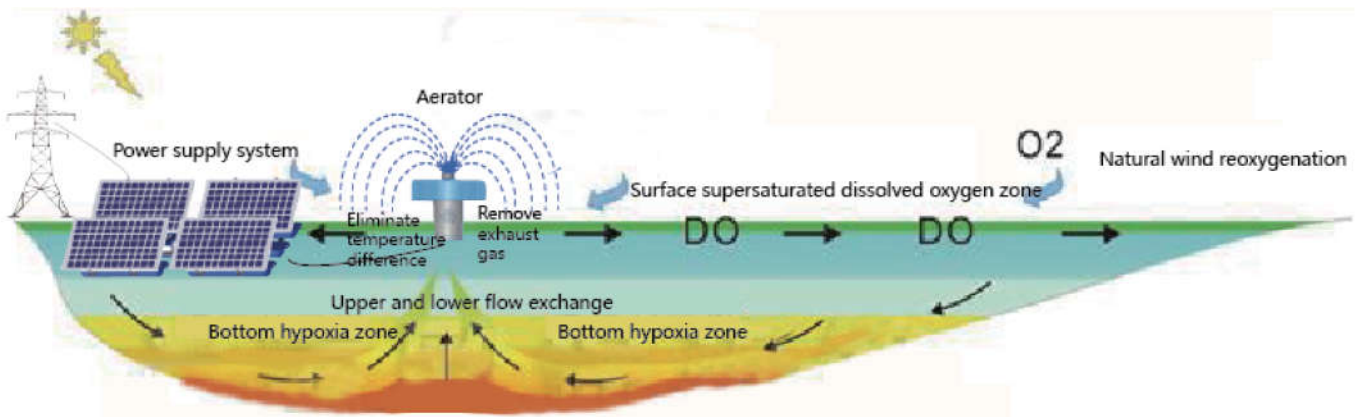
Schematic diagram of solar aeration system
